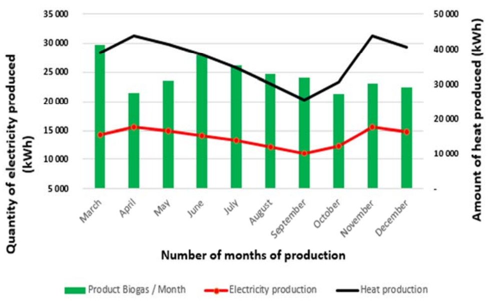
Figure 6. Energy production (heat and electricity) according to biogas in 2014.
